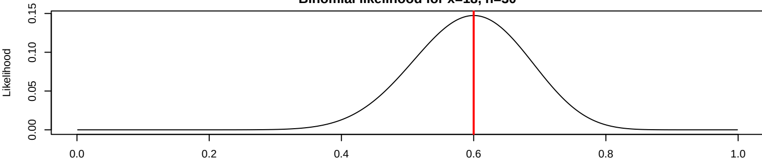
Binomial likelihood for x=18 , n=30
