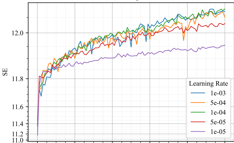
Training SE
