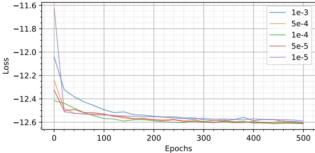
Validation Loss
