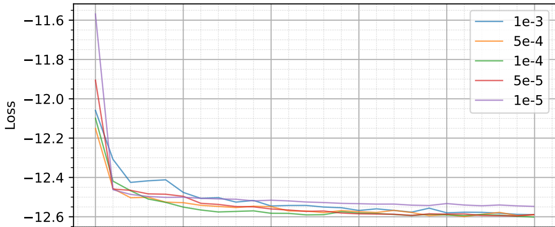
Training Loss
