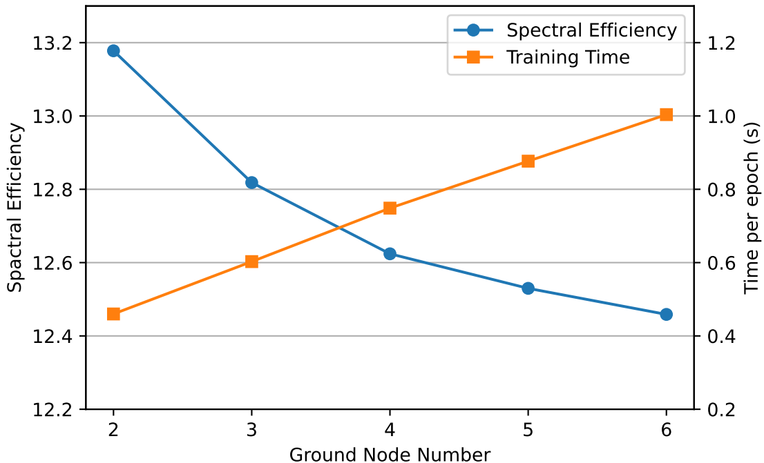
Spectral Efficiency and Training Time
