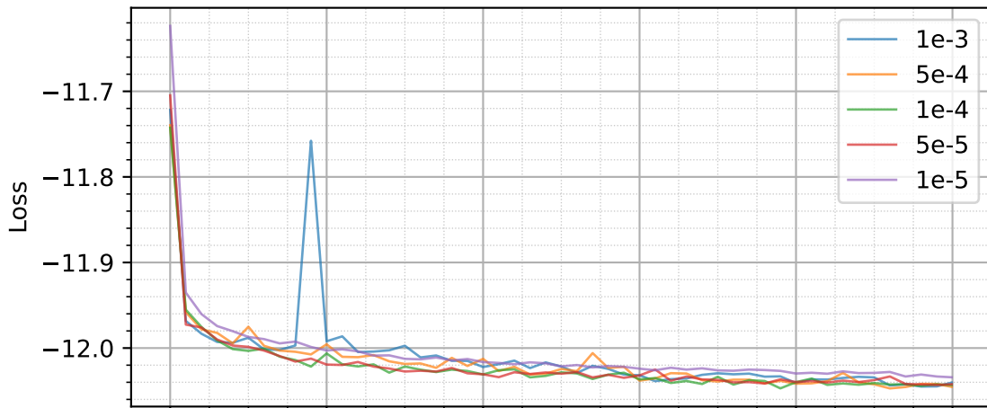
Training Loss
