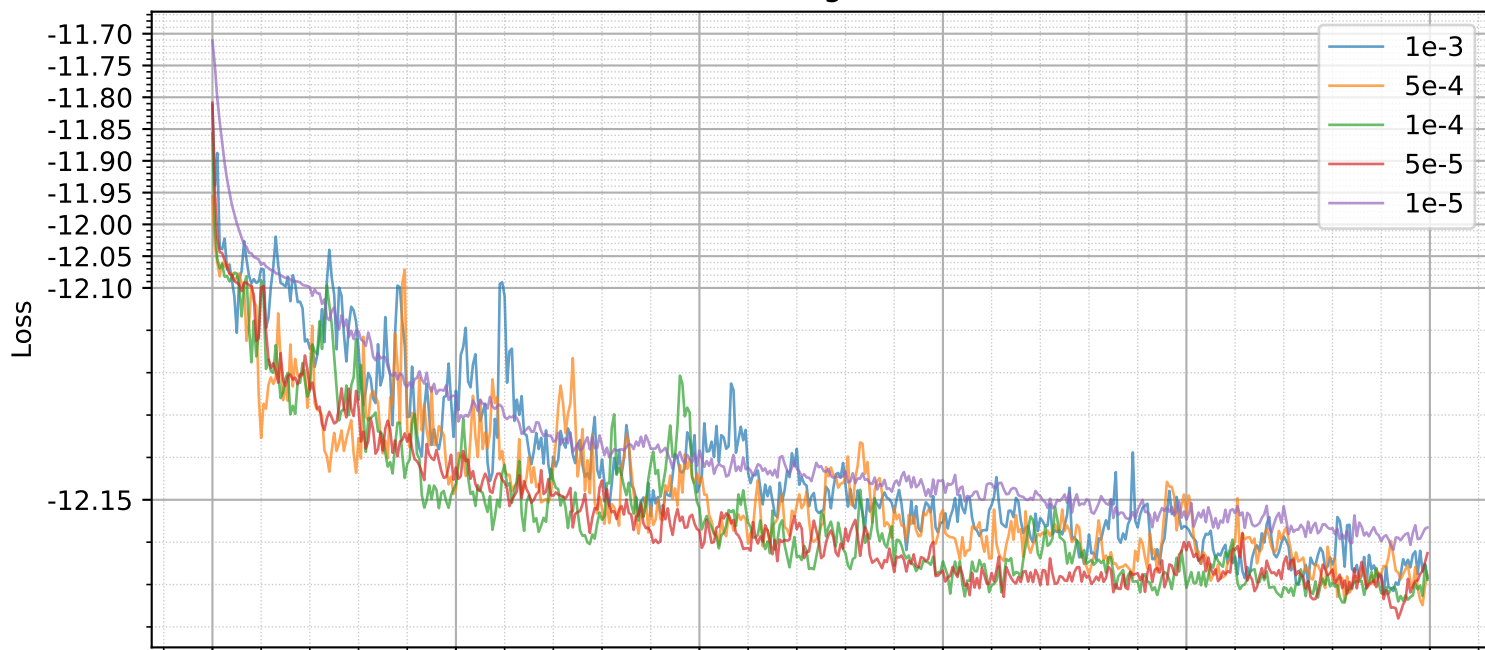
Validation Loss
