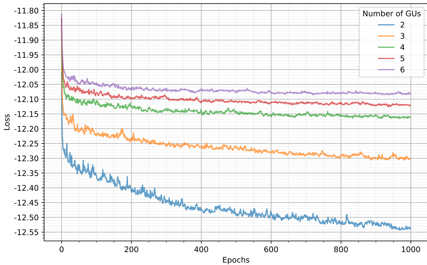
Validation Loss
