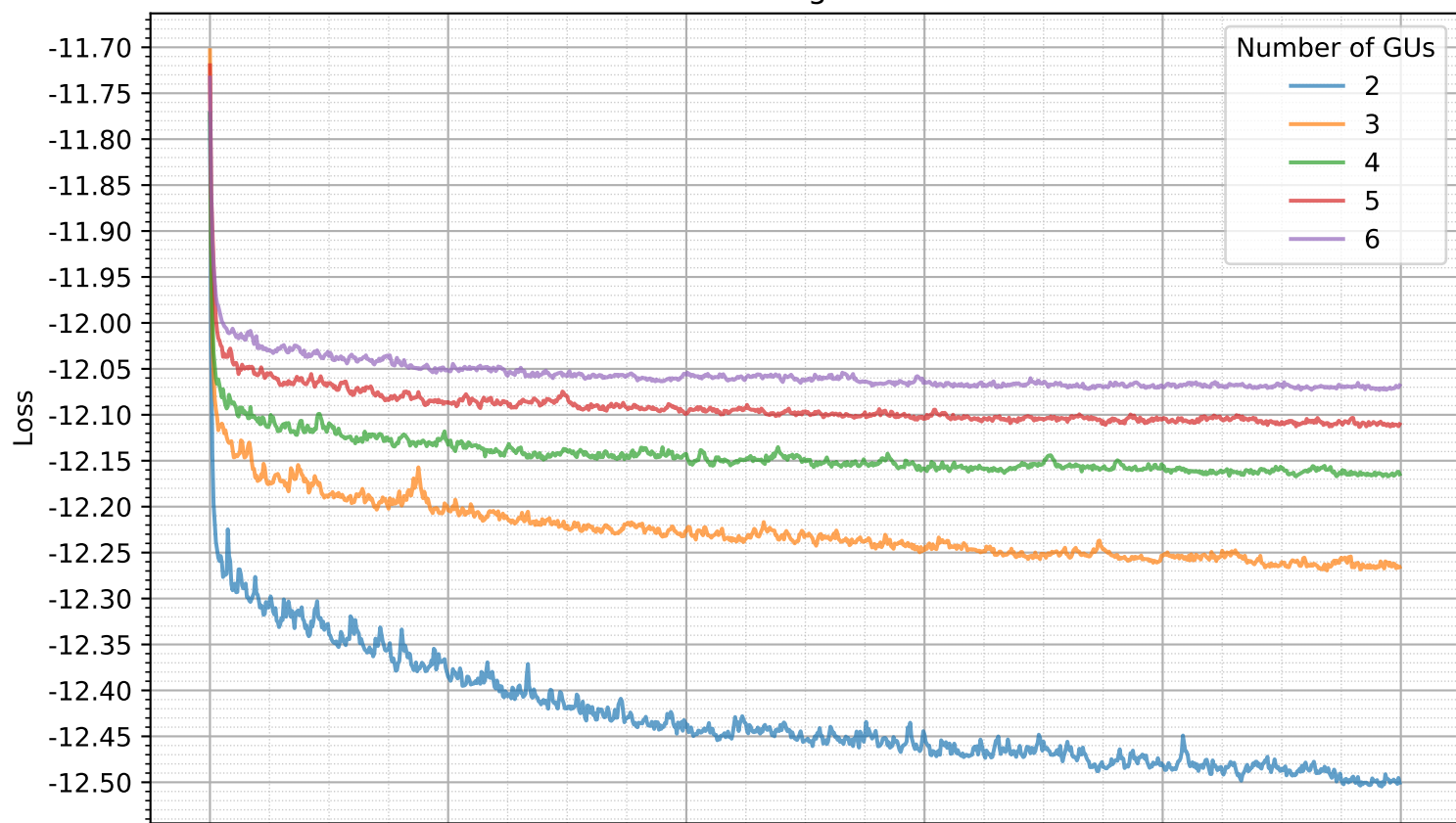
Training Loss
