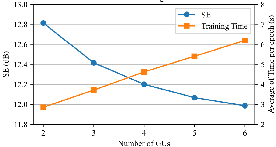
SE and Training Time
