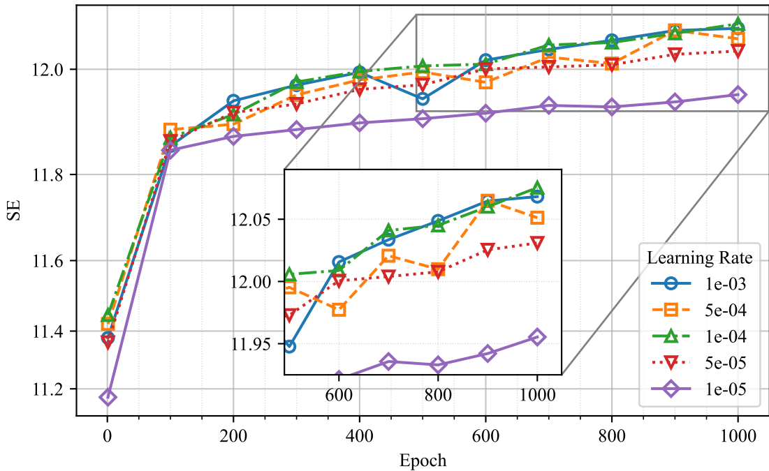
Training SE
