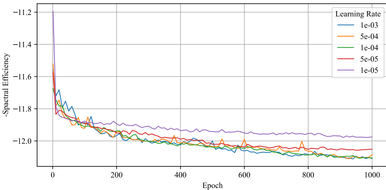
Validation Loss
