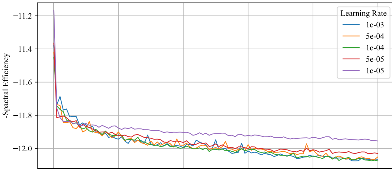
Training Loss
