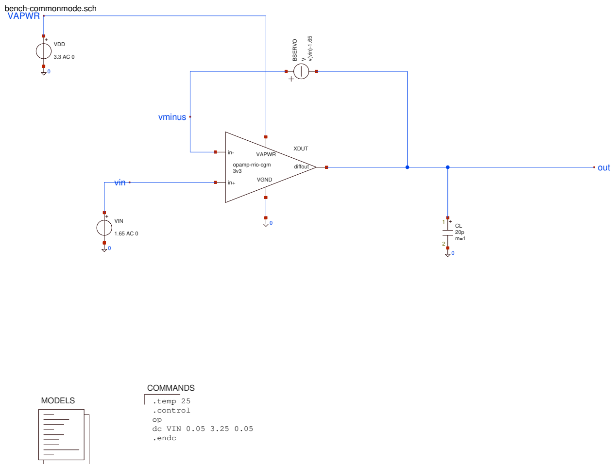
Figure 16. Native Xschem export of the common-mode testbench. BSERVO is a behavioral voltage source with V(\text{IN-}) - V(\text{OUT}) = V(\text{vin}) - 1.65 \text{ V} . Sweeping VIN moves both inputs while holding OUT near 1.65 V. It exists only in the testbench.
