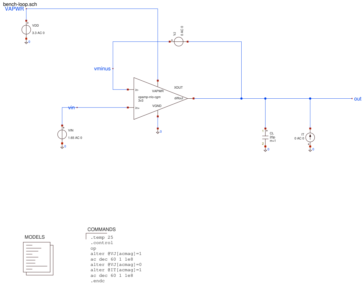
Figure 15. Native Xschem export of the two-injection loop testbench. VJ and IT are both zero at DC. The visible control block first excites VJ, then IT; VIN has AC = 0. Normal signal transfer is a third run with both injection stimuli zero and VIN AC = 1.
