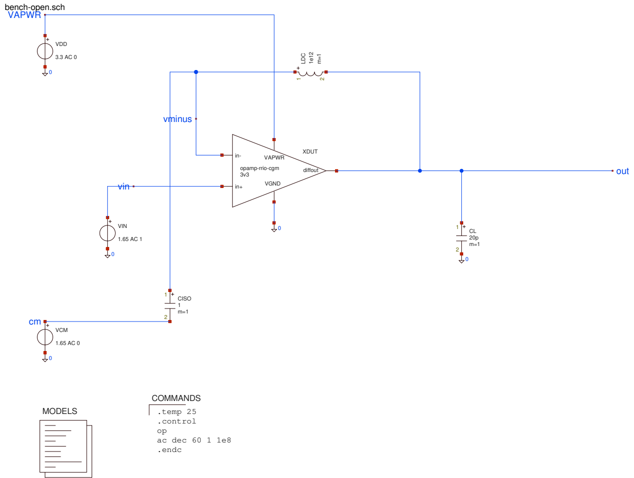
Figure 14. Native Xschem export of the open-loop voltage-gain testbench. LDC = 10^{12} \text{ H} preserves DC feedback; CISO = 1 \text{ F} holds IN- at AC ground through VCM = 1.65 \text{ V} , AC = 0 . These are ideal testbench devices. The source labels and connections match the documented gain measurement.
