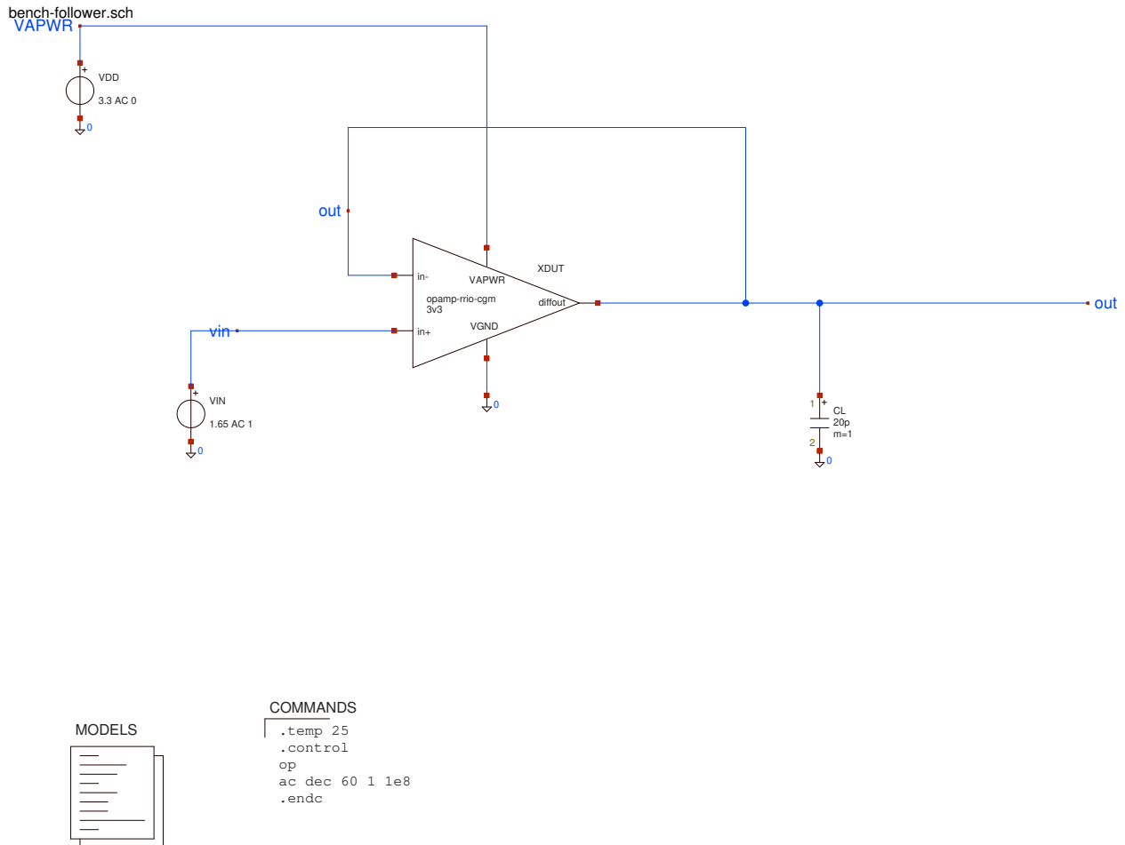
Figure 13. Native Xschem export of the follower testbench, using the project's OpAmp symbol, an explicit 3.3 V source and 20 pF load. The shown source setting is for signal AC; transient tests replace VIN's stimulus with the stated step waveform. Direct OUT-to-IN- feedback is correct for both.
