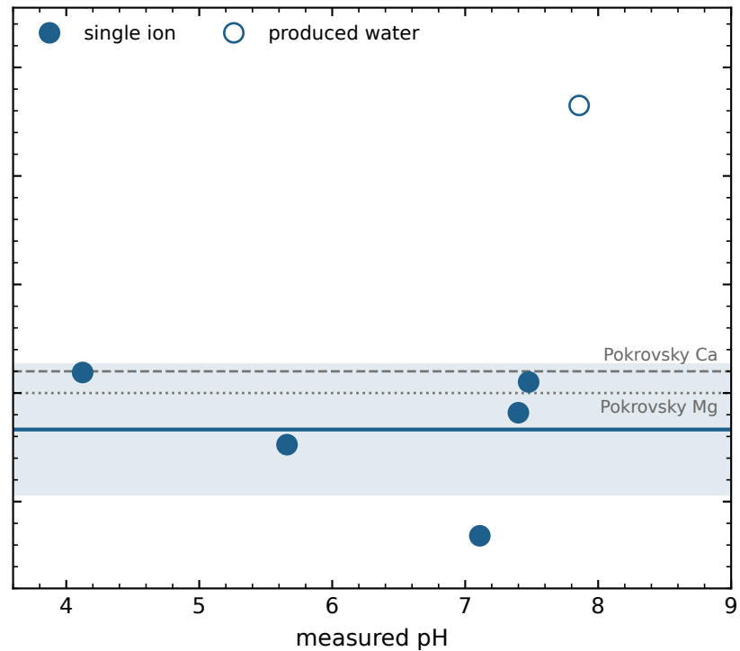
Co single ion mean -2.34 \pm 0.61
