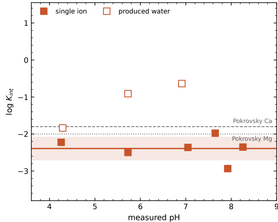
Li single ion mean -2.39 \pm 0.32
