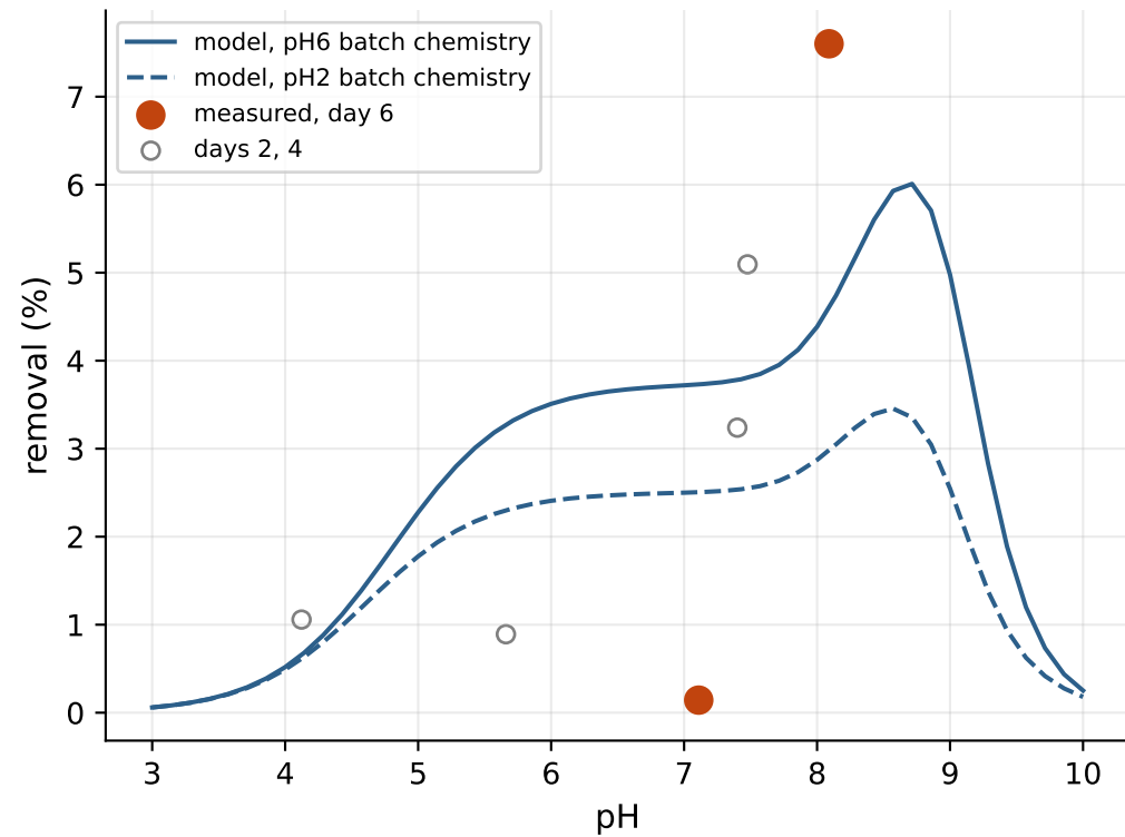
Figure 2 Co adsorption edge (log K = -2.18)
