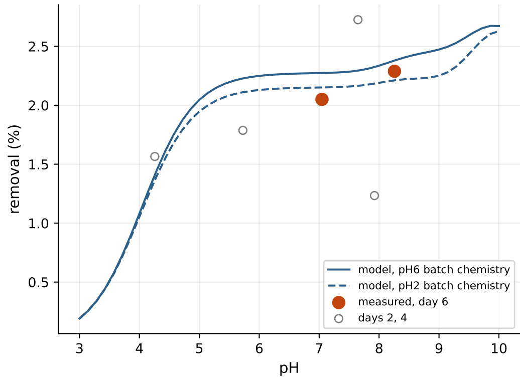
Figure 2 Li adsorption edge (log K = -2.31)
