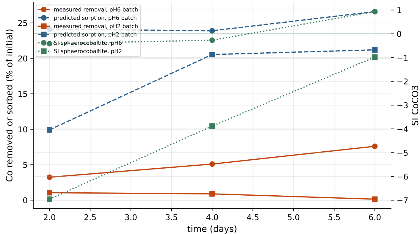
Step 8 Cobalt: measured removal vs predicted sorption, with saturation index
