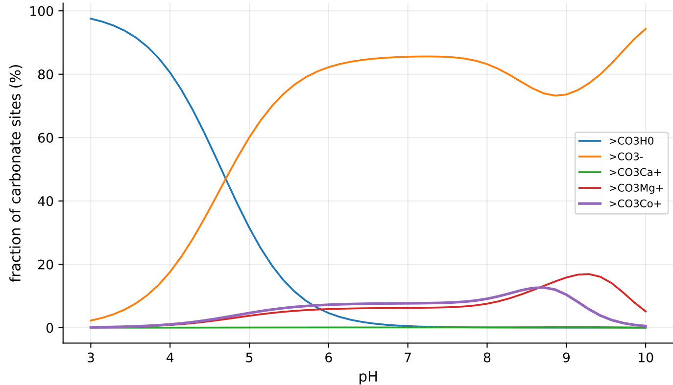
Carbonate-site speciation, Co batch chemistry (Ca 0.13, Mg 12.9 ppm)
