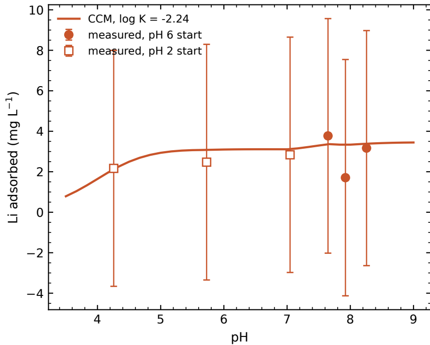
Li adsorption envelope
