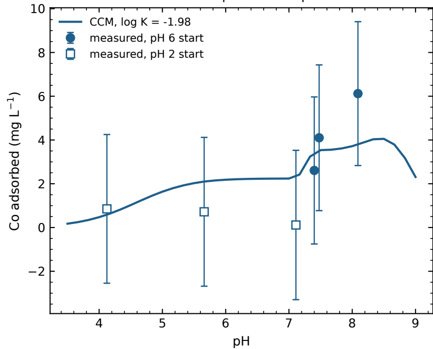
Co adsorption envelope
