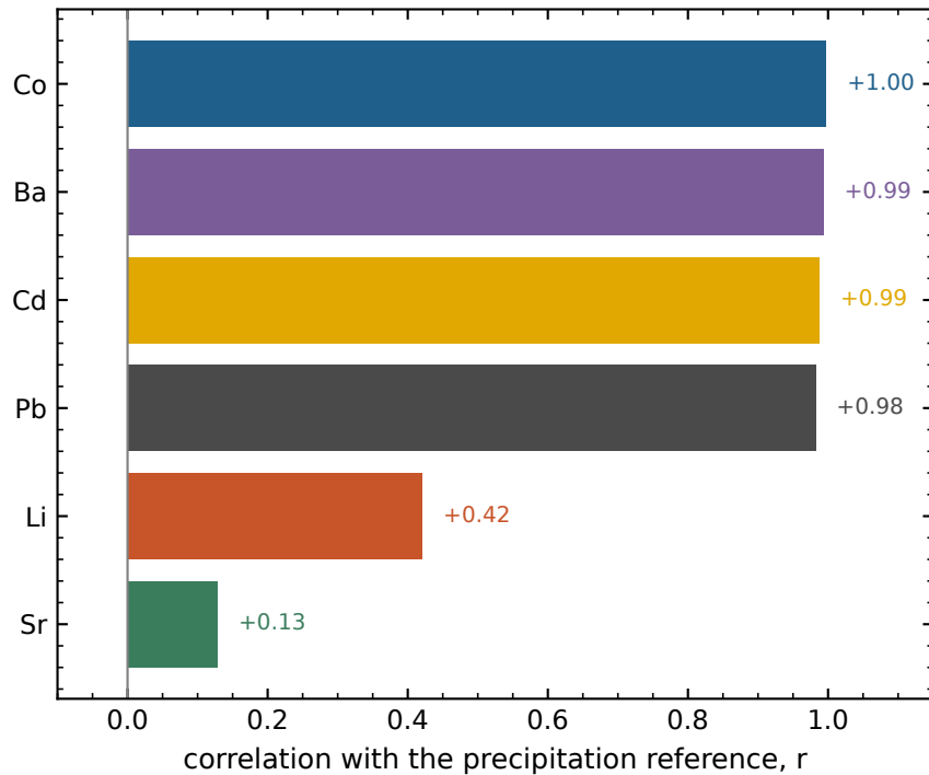
Sr and Li separate; Ba does not
