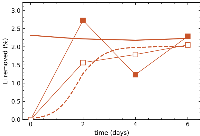
(C) Li, produced water — \log K_{int} = -1.13
