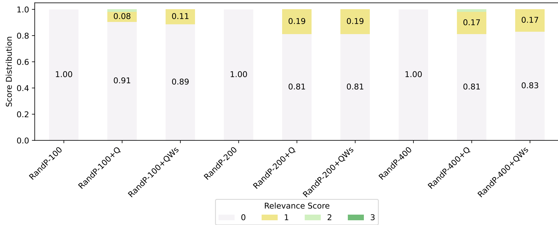
GPT-3.5-turbo - Basic
