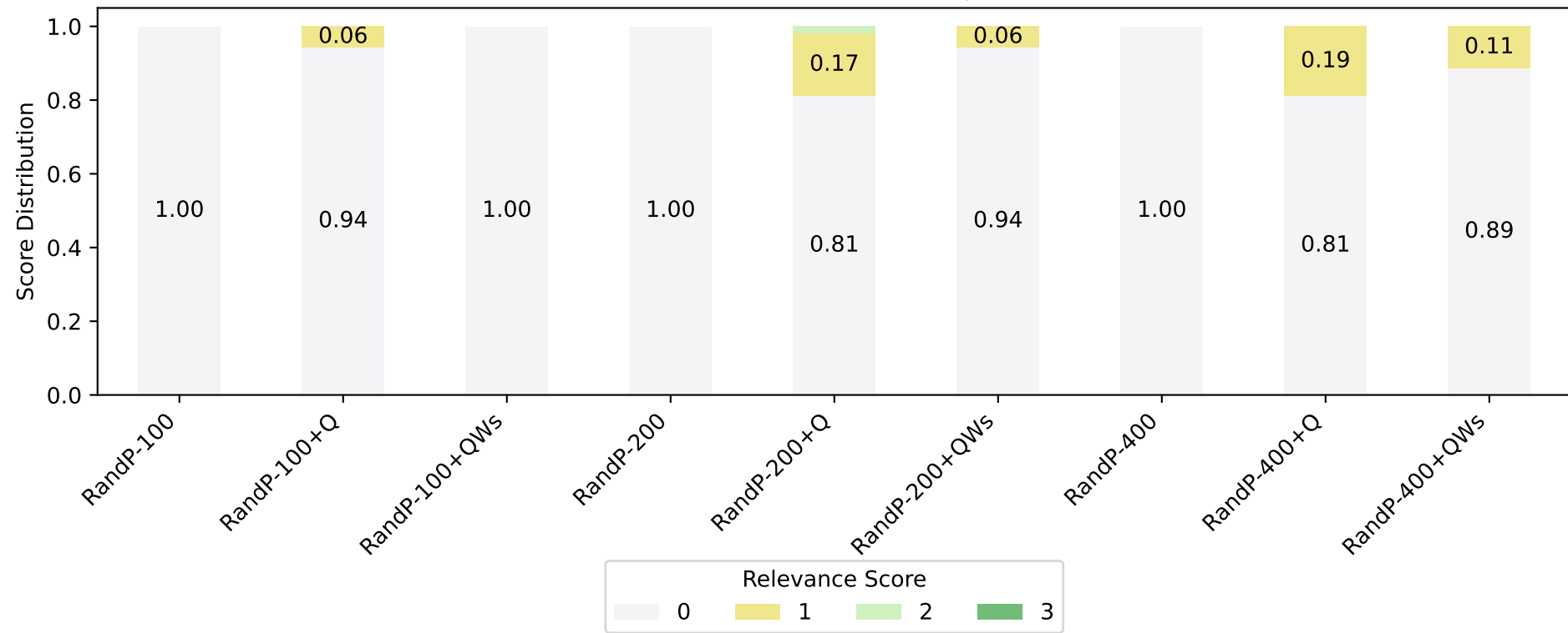
GPT-3.5-turbo - Utility
