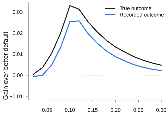
A. Errors unrelated to risk (Se 0.85, Sp 0.98)
