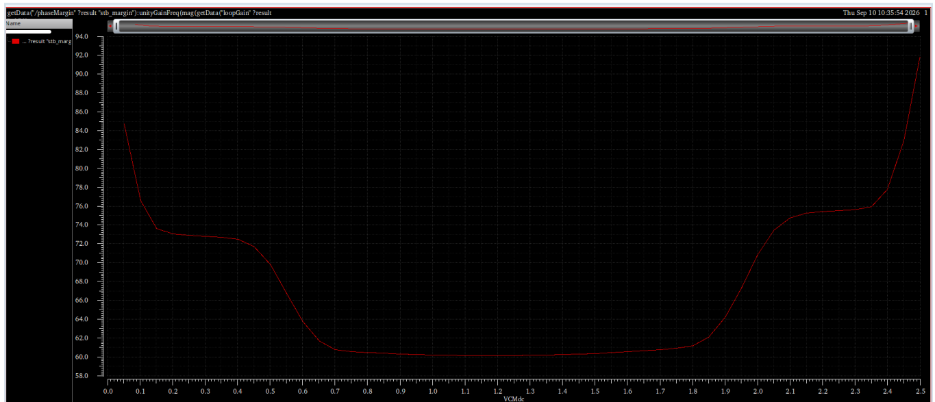
Figure 5. Phase margin versus common-mode voltage for the captured sweep; the visible minimum is approximately 60.1 to 60.2 degrees.
