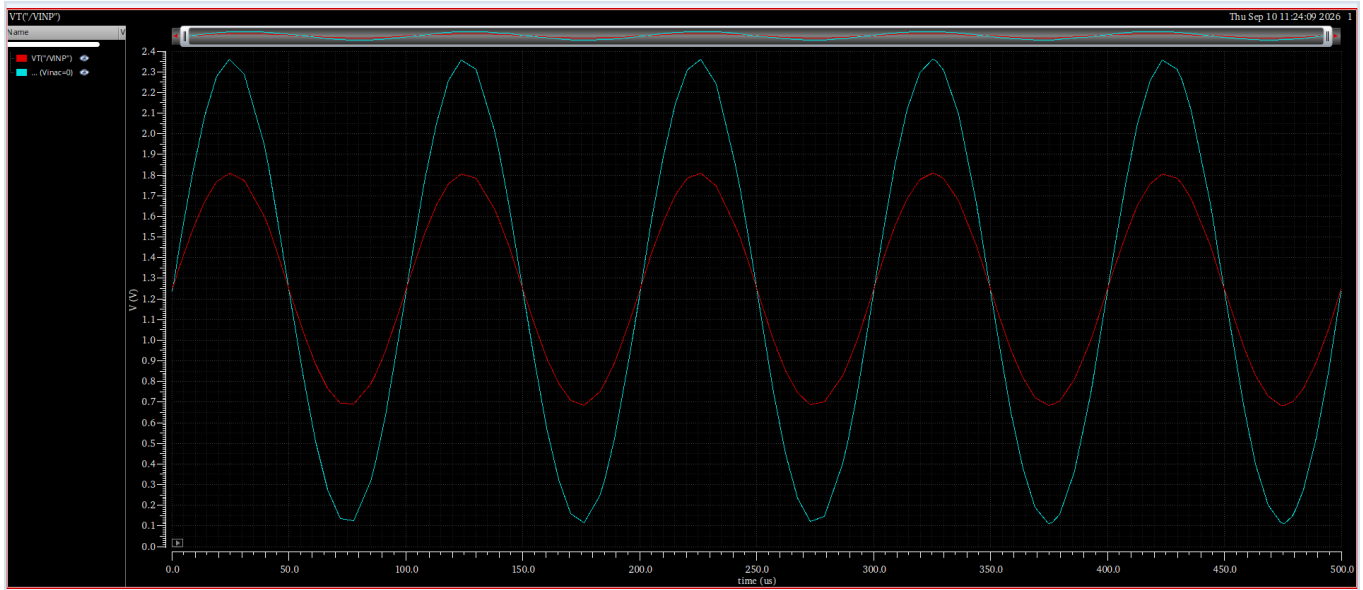
Figure 11. TB2, non-inverting gain +2, at 10 kHz. Approximate input span: 0.69 to 1.80 V; output: 0.11 to 2.36 V.
