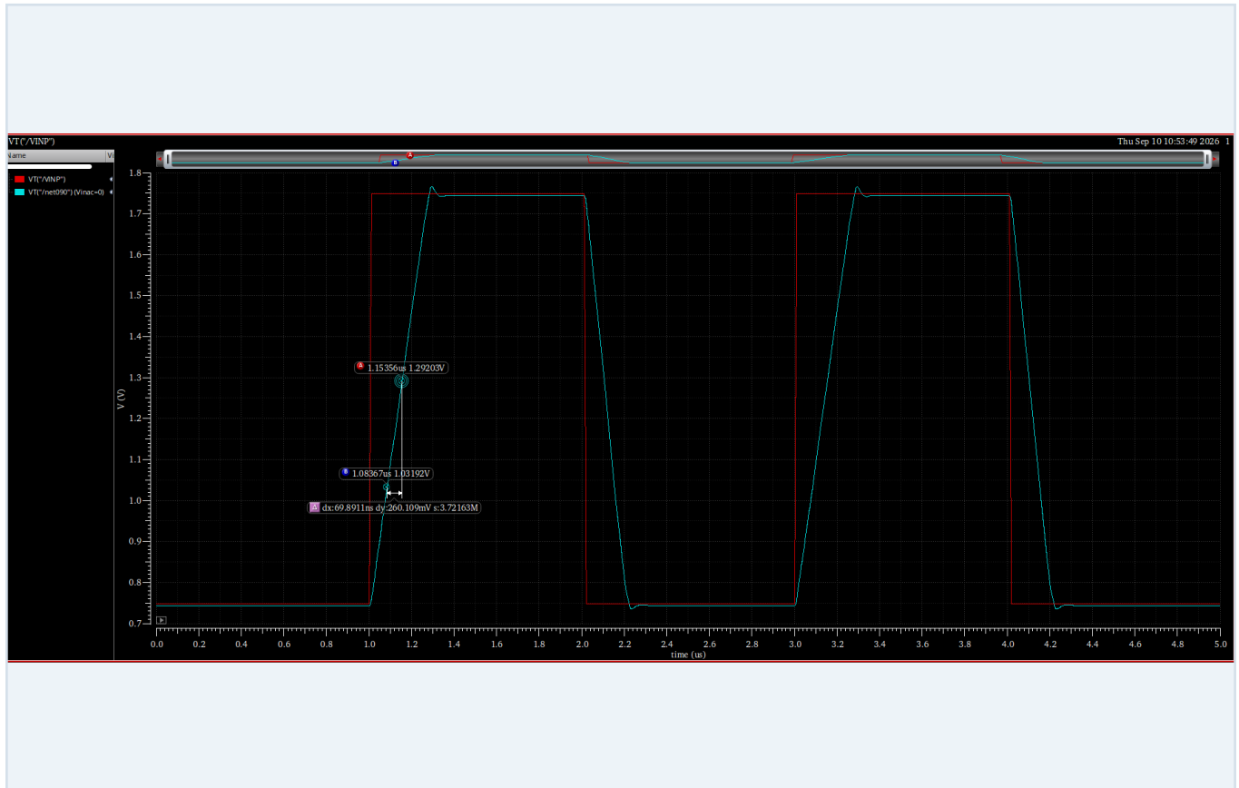
Figure 10. Unity-buffer step response with a positive-slope measurement of approximately 3.72 V/us.
