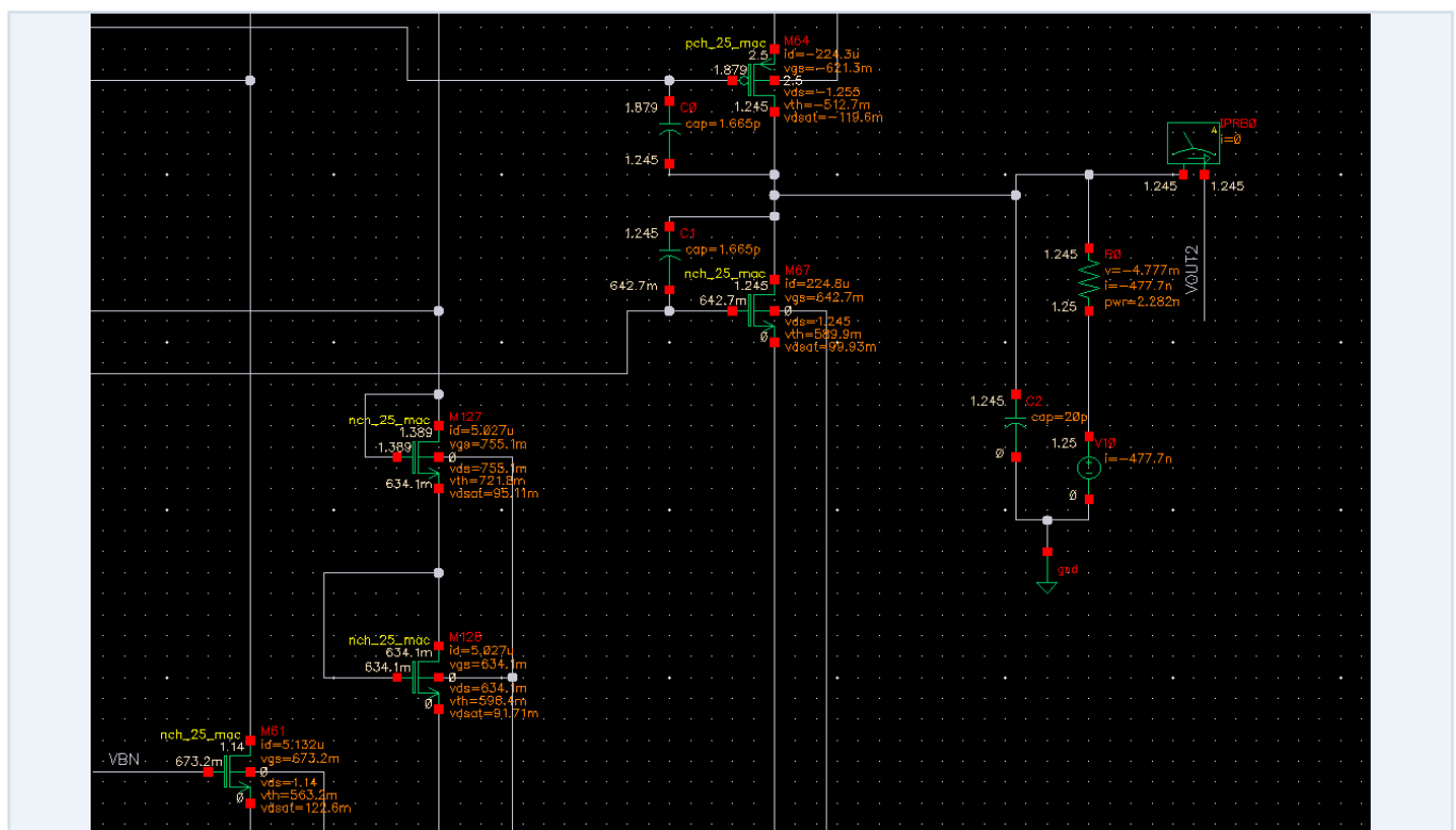
Figure 1. Annotated output stage and load. The implemented devices are M64 (PMOS) and M67 (NMOS). V_{OUT} is approximately 1.245 V.
