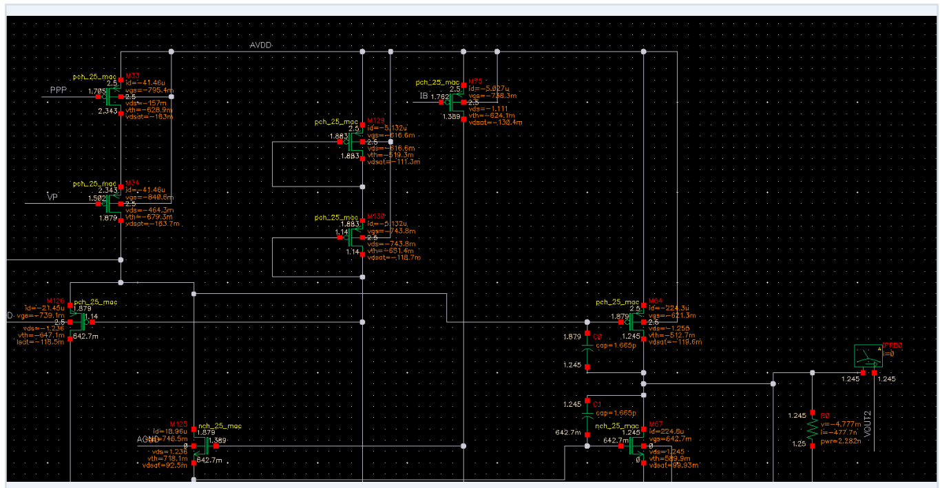
Figure 2. Additional annotated local operating-point view from the implemented amplifier. Original device names and annotations are retained.
