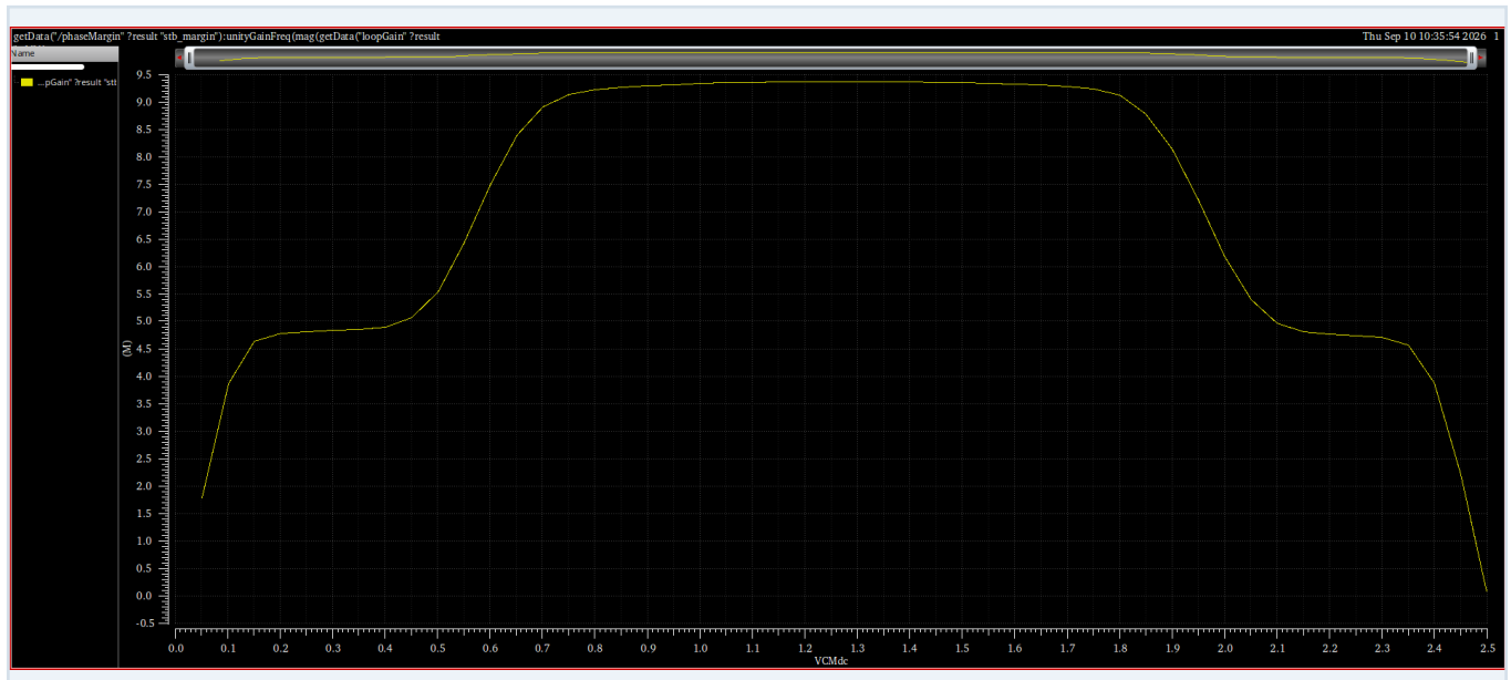
Figure 4. Unity-gain frequency, f_u , versus input common-mode voltage. This is not gain-bandwidth product.
