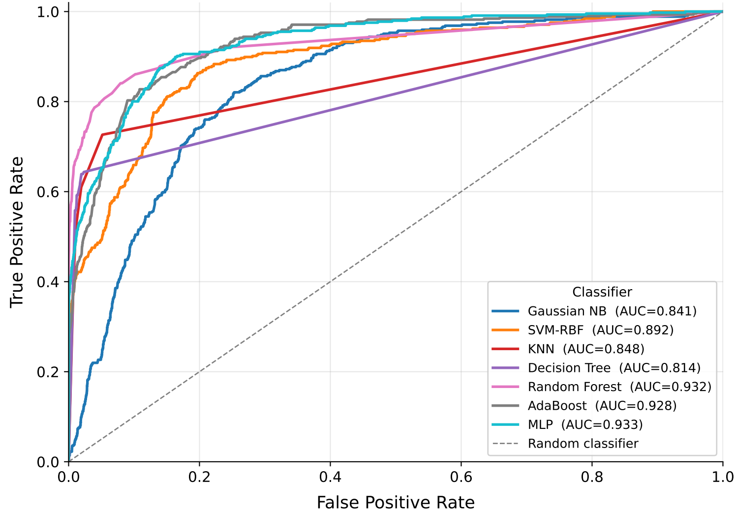
ROC Curves — Aggregated Out-of-Fold Predictions (5-Fold CV)
