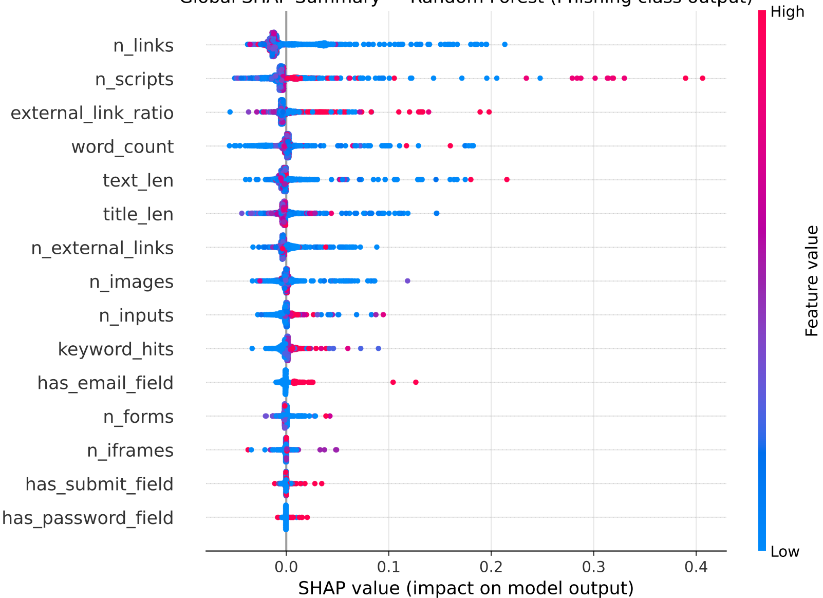
Global SHAP Summary — Random Forest (Phishing class output)
