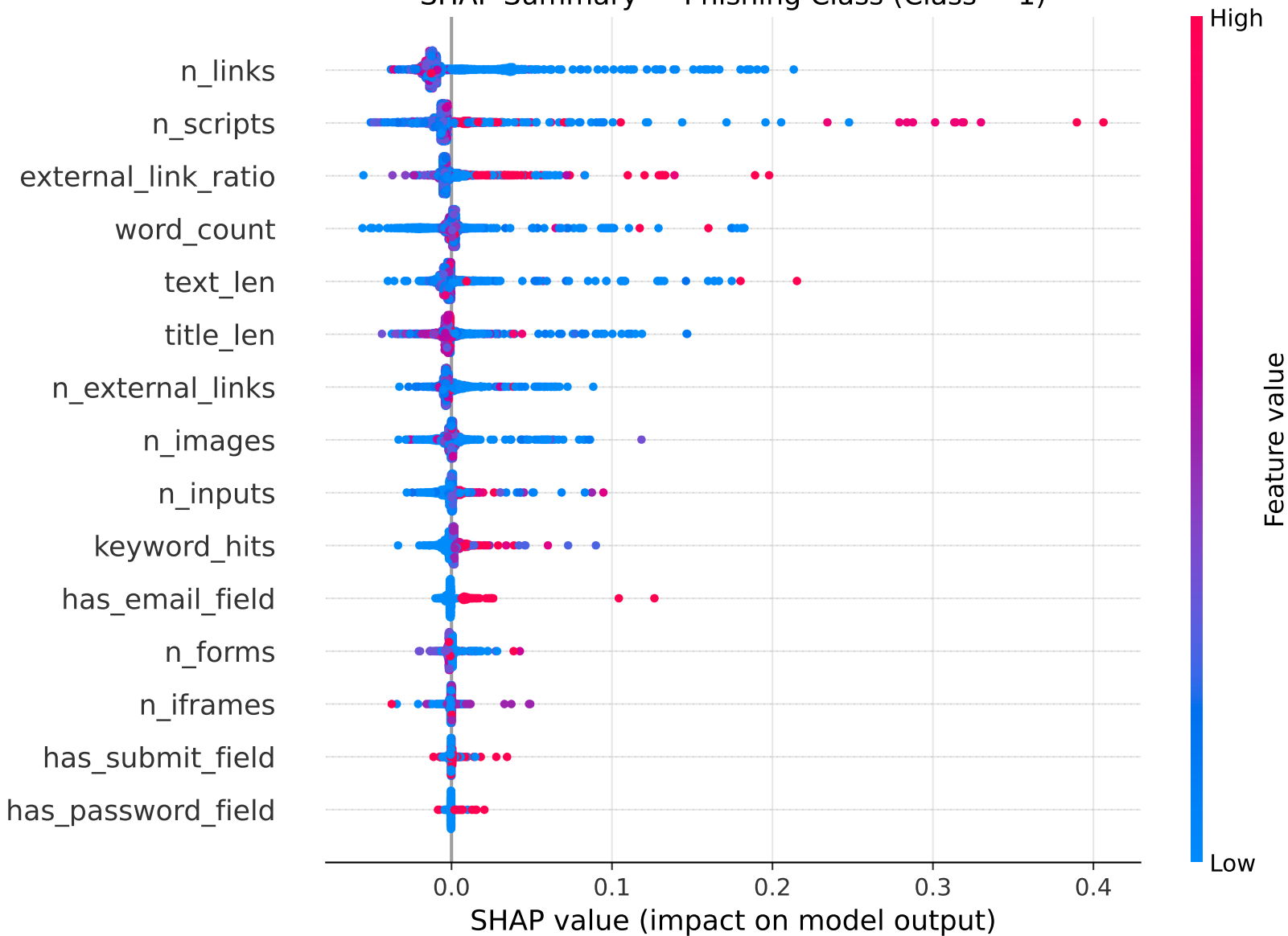
SHAP Summary — Phishing Class (Class = 1)
