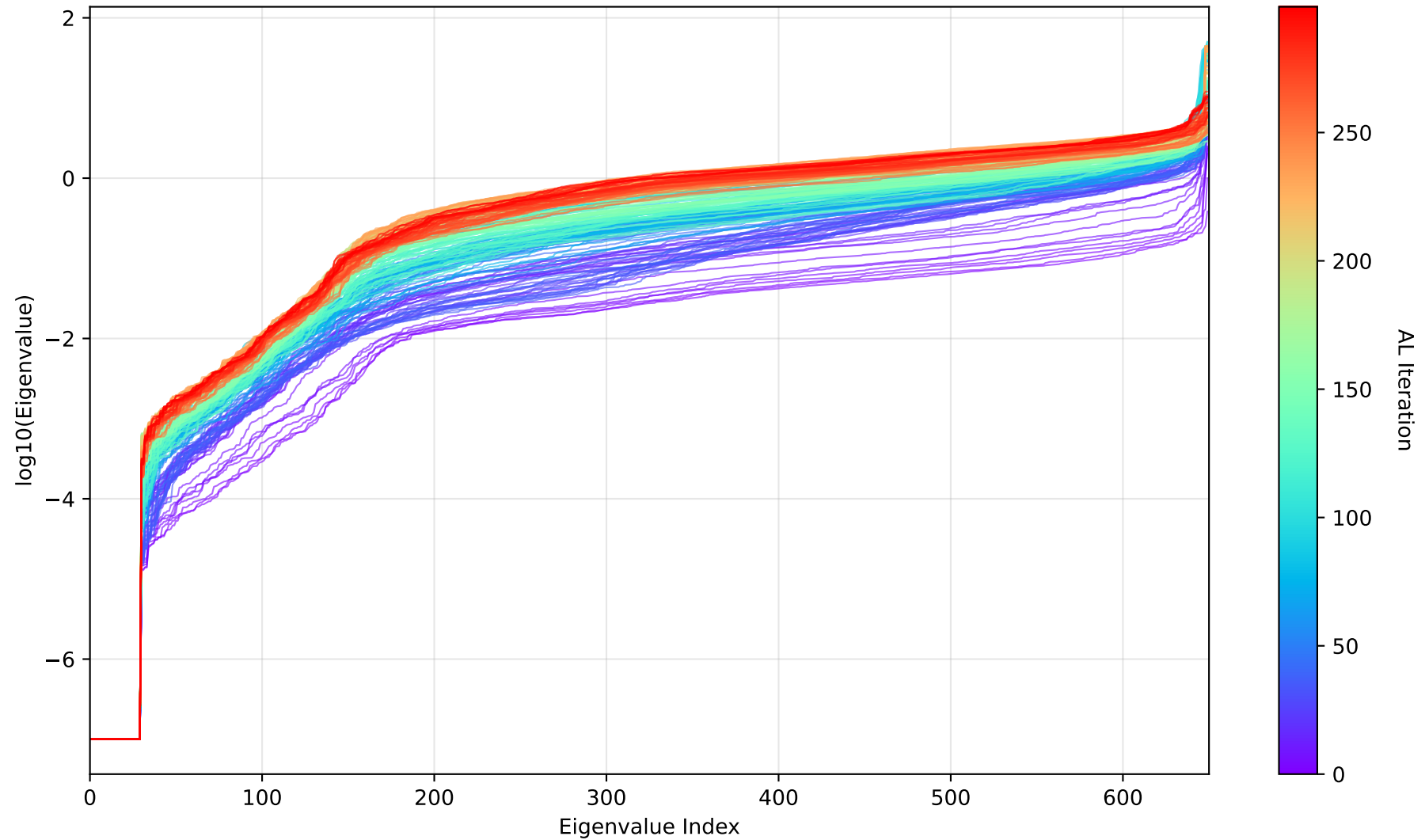
Hessian Eigenvalue Distribution Evolution (A-opt)
