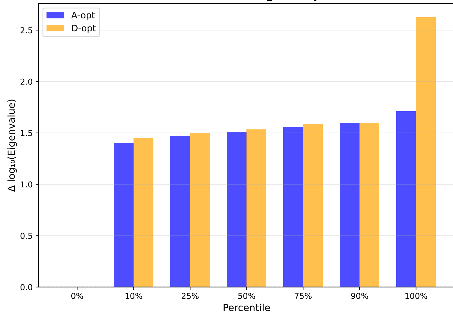
Percentile-wise Change Comparison
