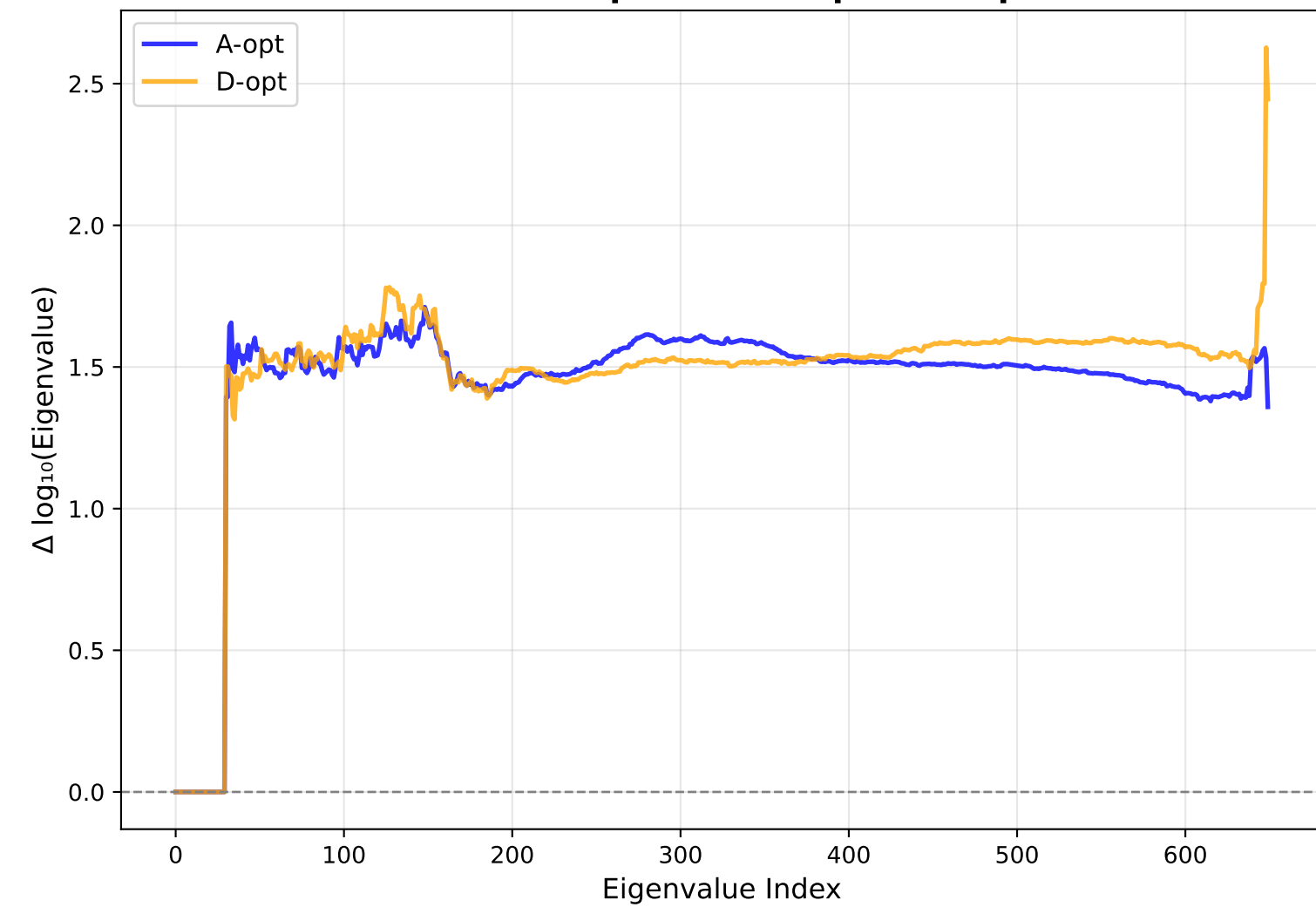
Direct Comparison: A-opt vs D-opt
