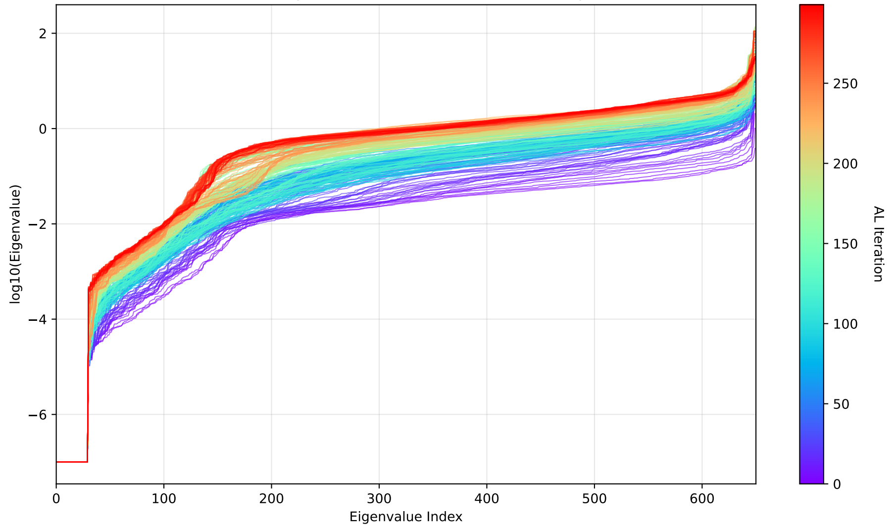
Hessian Eigenvalue Distribution Evolution (T-opt)
