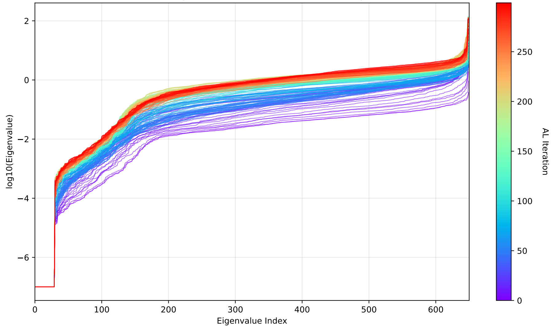
Hessian Eigenvalue Distribution Evolution (D-opt)
