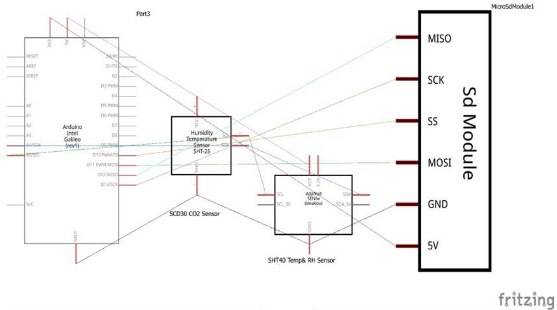
Figure 2. System wiring schematic showing the electrical connections between the Arduino, SCD30 sensor, SHT40 sensor, and microSD card module.
