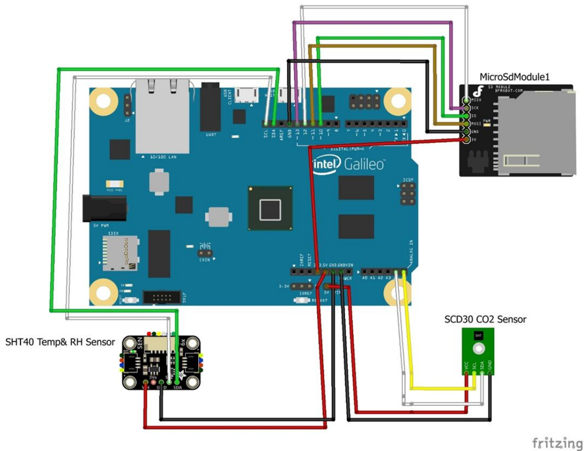
Figure 1. Physical wiring diagram of the Arduino based monitoring system
