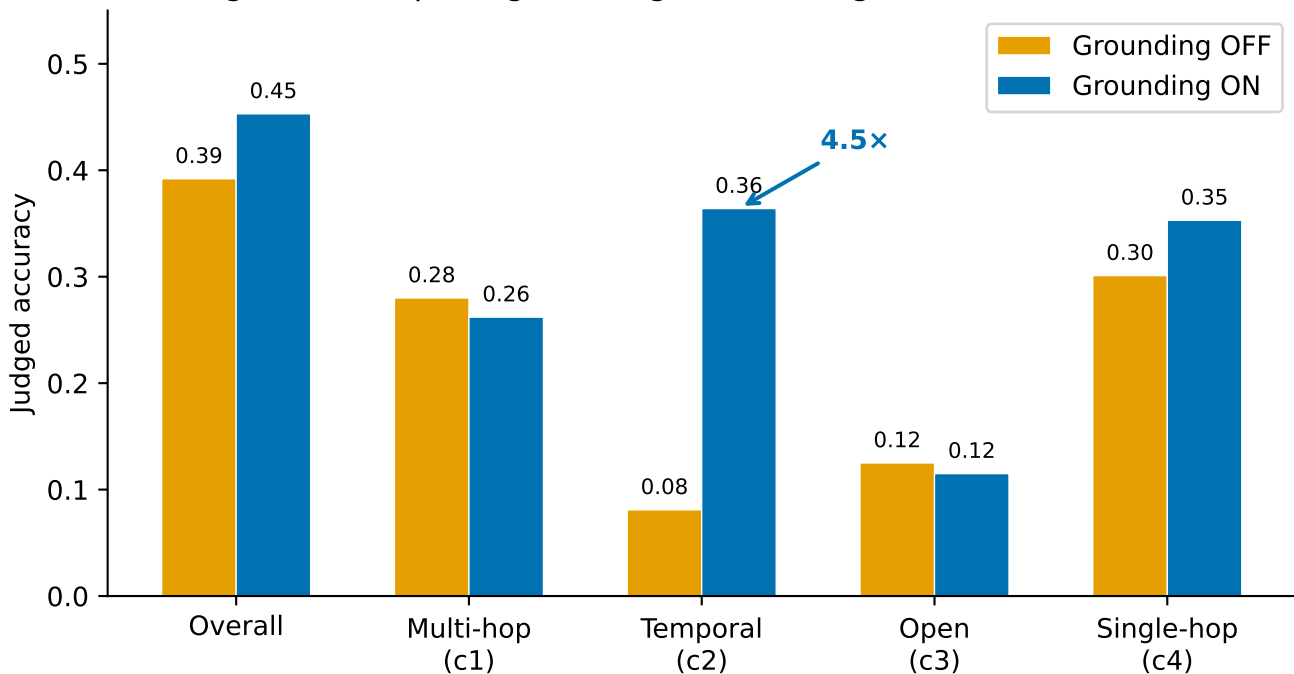
Figure 3: Temporal grounding ablation (agentic, Gemma4-12B)
