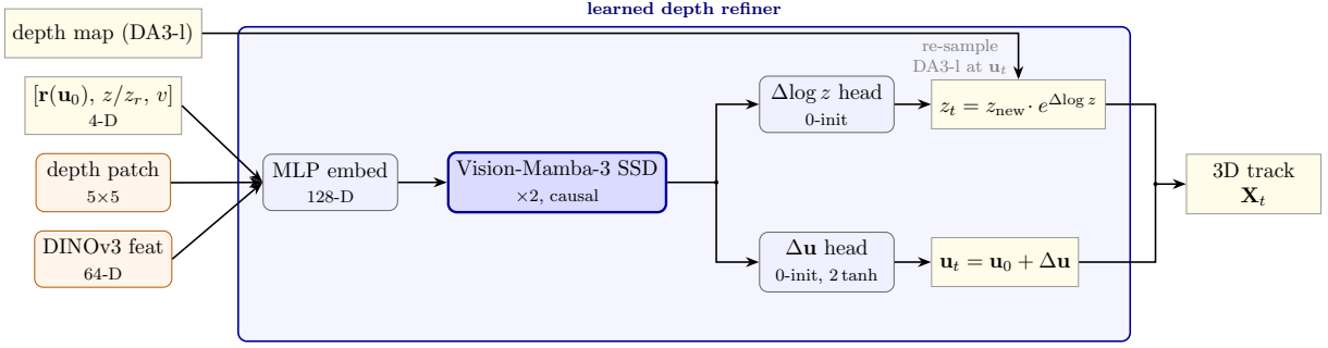
Figure 5: v35 architecture (extends Fig. 3) — again the inside of the blue box in Fig. 1. Orange nodes are new relative to v33. \mathbf{u}_0 is the 2-D pixel position from SEA-RAFT optical flow (Fig. 6); it determines the ray direction \mathbf{r}(\mathbf{u}_0) , the centre of the 5 \times 5 depth patch, and the location at which the DINOv3 feature is sampled. All three inputs are concatenated, embedded by the MLP, and then fed through the Vision-Mamba-3 SSD layers (the same causal SSD stack as v33’s Mamba-3, but now conditioned on DINOv3 appearance — which is exactly what makes it Vision -Mamba-3 rather than the geometry-only Mamba-3 of v33). A second head produces \Delta \mathbf{u} = 2 \tanh(\cdot) (bounded to \pm 2 px). Depth is then re-sampled at the corrected pixel \mathbf{u}_t = \mathbf{u}_0 + \Delta \mathbf{u} from the DA3-l depth map, and \Delta \log z rescales it. Both heads are zero-initialised: v35 starts exactly at the v33 output.
