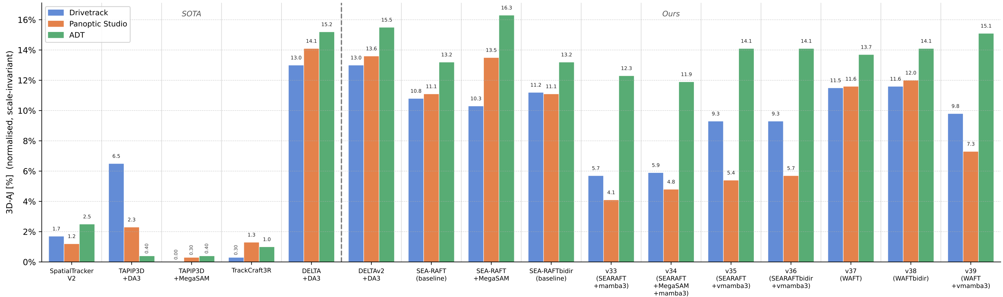
TAPVid-3D Normalised Median-AJ (leaderboard metric, higher = better)
