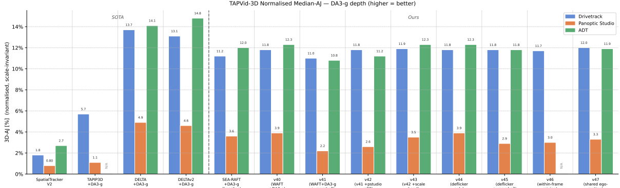
Figure 12: Method comparison on DA3-g depth, normalised median-AJ (leaderboard, scale-invariant; higher better), for the methods that consume DA3-g. TAPIP3D adt is OOM-limited (“N/A”). Cf. the DA3-l version, Fig. 10.
