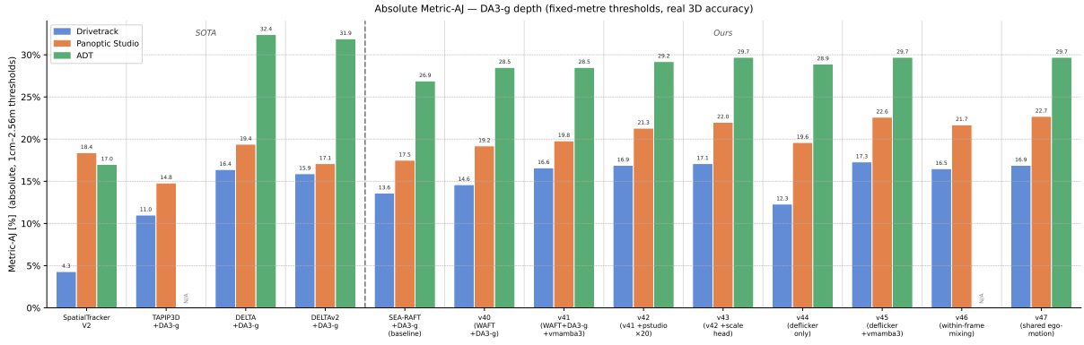
Figure 13: Method comparison on DA3-g depth, absolute metric-AJ (fixed-metre thresholds; higher better). Drivetrack rises across the board vs. DA3-l (Fig. 11), but pstudio/adl do not, so even v42 — our best DA3-g pipeline (mean 0.225), which adds a pstudio \times 20 near-boost over v41 — does not beat the DA3-l v39 overall (0.246). TAPIP3D adt is OOM-limited (“N/A”).
