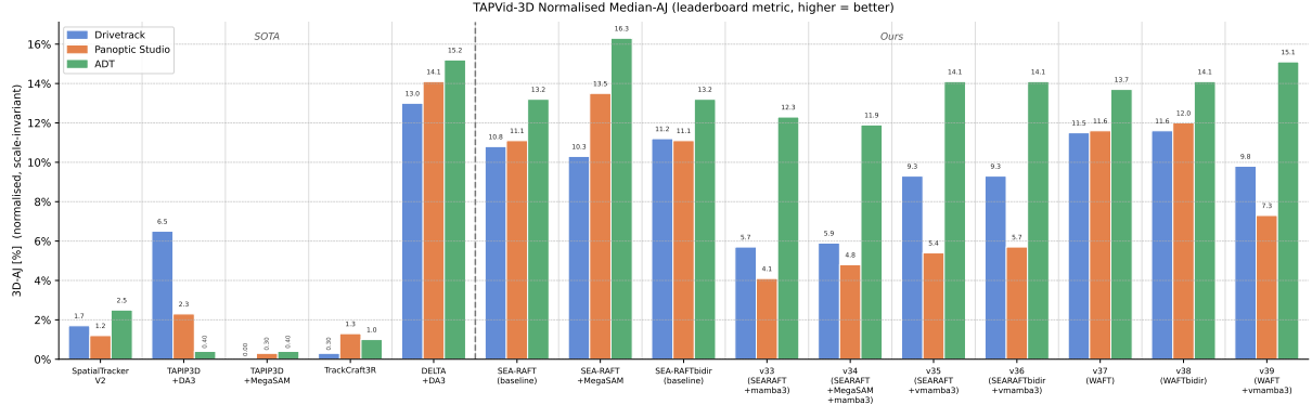
Figure 9: Method comparison on TAPVid-3D minival, normalised median-AJ (leaderboard metric, scale-invariant). Higher is better. “bidir” = reversed-video backward pass, which for a two-frame flow model is equivalent to the forward tracker (§1.8), so the “bidir” bars match their non-bidir counterparts up to run-to-run nondeterminism. TrackCraft3R’s low drivetrack bar reflects an OOD failure (see §2.4).
