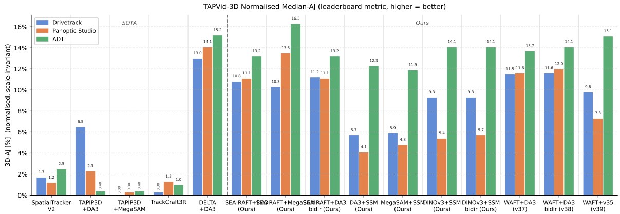
Figure 8: Method comparison on TAPVid-3D minival, normalised median-AJ (leaderboard metric, scale-invariant). Higher is better. “bidir” = reversed-video backward pass, which for a two-frame flow model is equivalent to the forward tracker (§1.7), so the “bidir” bars match their non-bidir counterparts up to run-to-run nondeterminism. TrackCraft3R’s low drivetrack bar reflects an OOD failure (see §2.4).
