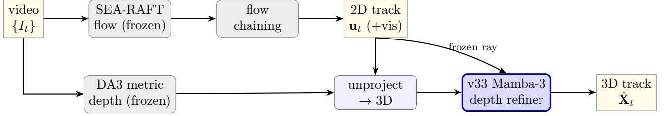
Figure 1: Pipeline. Grey = frozen / training-free; blue = the only learned module (0.40M params). The 2D track and visibility from SEA-RAFT are never modified; v33 refines depth along each point’s fixed pixel ray, so the 2D reprojection is invariant by construction (Fig. 2).
