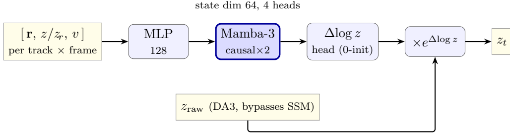
Figure 3: v33 architecture. Input abbreviations: \mathbf{r}=(\text{ray}_x, \text{ray}_y) , z/z_r=z_{\text{raw}}/z_{\text{ref}} , v =visibility. Bypass: z_{\text{raw}} (DA3 metric depth) skips the SSM entirely and is multiplied back in at the end — the SSM is a relative corrector that predicts the factor e^{\Delta \log z} , not an absolute depth. causal \times 2 : two causal Mamba-3 layers (past-only; enables streaming). 4 heads: SSD splits the 64-dim state into 4 independent heads (16-dim each), analogous to multi-head attention but computed as a linear recurrence.
