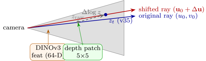
New SSM inputs (orange/green) \Rightarrow informed \Delta \mathbf{u} avoids depth-discontinuity artefacts. Depth is re-sampled at \mathbf{u}_0 + \Delta \mathbf{u} before applying \Delta \log
