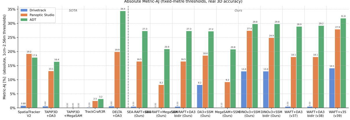
Figure 9: Same methods, absolute metric-AJ (fixed-metre thresholds 1 cm–2.56 m; higher better). v39 (WAFIT flow + v35 refiner) leads all methods, ahead of the SEA-RAFT-fed v35, despite both ranking below SEA-RAFT+MegaSAM on the leaderboard metric.
