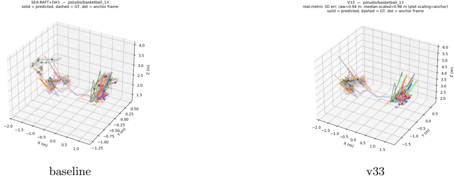
Figure 12: pstudio (indoor, \sim 3 m): 3D trajectories, baseline vs v33.
