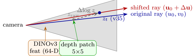
Figure 4: v35 joint correction. Two new inputs (DINOv3 appearance features and a local 5 \times 5 depth patch) give the SSM the context needed to predict \Delta \mathbf{u} safely. Unlike v32, which nudged the pixel blindly and crossed depth discontinuities, v35’s 2D correction is conditioned on local appearance and local depth structure. Depth is re-sampled at the shifted pixel before e^{\Delta \log z} rescales it.
