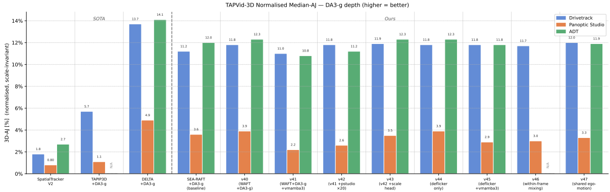
Figure 12: Method comparison on DA3-g depth, normalised median-AJ (leaderboard, scale-invariant; higher better), for the methods that consume DA3-g. TAPIP3D adt is OOM-limited (“N/A”). Cf. the DA3-l version, Fig. 10.
