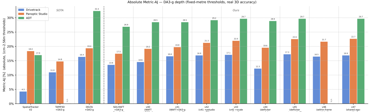
Figure 13: Method comparison on DA3-g depth, absolute metric-AJ (fixed-metre thresholds; higher better). Drivetrack rises across the board vs. DA3-l (Fig. 11), but pstudio/adl do not, so even v42 — our best DA3-g pipeline (mean 0.225), which adds a pstudio \times 20 near-boost over v41 — does not beat the DA3-l v39 overall (0.246). TAPIP3D adt is OOM-limited (“N/A”).
