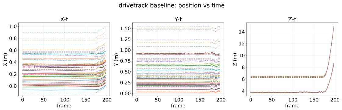
Figure 17: Space-time view (drivetrack baseline): per-axis position over time, X - t / Y - t / Z - t , predicted (solid) vs ground truth (dashed).
