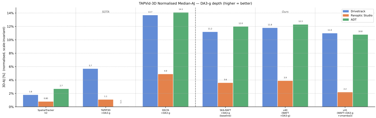
Figure 10: Method comparison on DA3-g depth, normalised median-AJ (leaderboard, scale-invariant; higher better), for the methods that consume DA3-g. TAPIP3D adt is OOM-limited (“N/A”). Cf. the DA3-1 version, Fig. 8.
