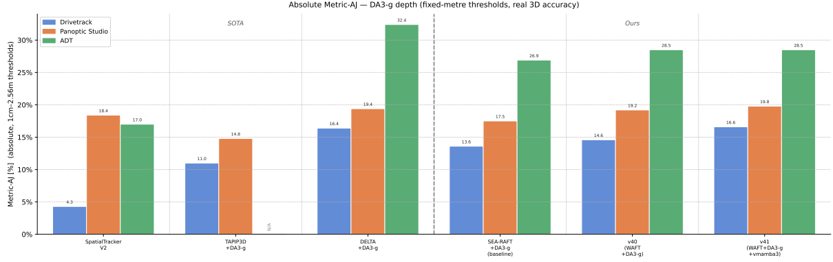
Figure 11: Method comparison on DA3-g depth, absolute metric-AJ (fixed-metre thresholds; higher better). Drivetrack rises across the board vs. DA3-l (Fig. 9), but pstudio/adtt do not, so v41 does not beat the DA3-l v39 overall. TAPIP3D adtt is OOM-limited (“N/A”).
