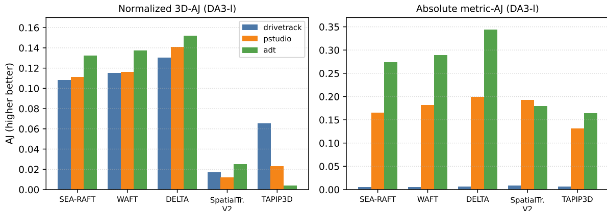
Figure 7: External baselines on DA3-l depth, per subset: normalized 3D-AJ (left) and absolute metric-AJ (right). Metric-AJ on drivetrack is near-zero for every direct-unprojection method (the DA3-l far-field scale collapse).
