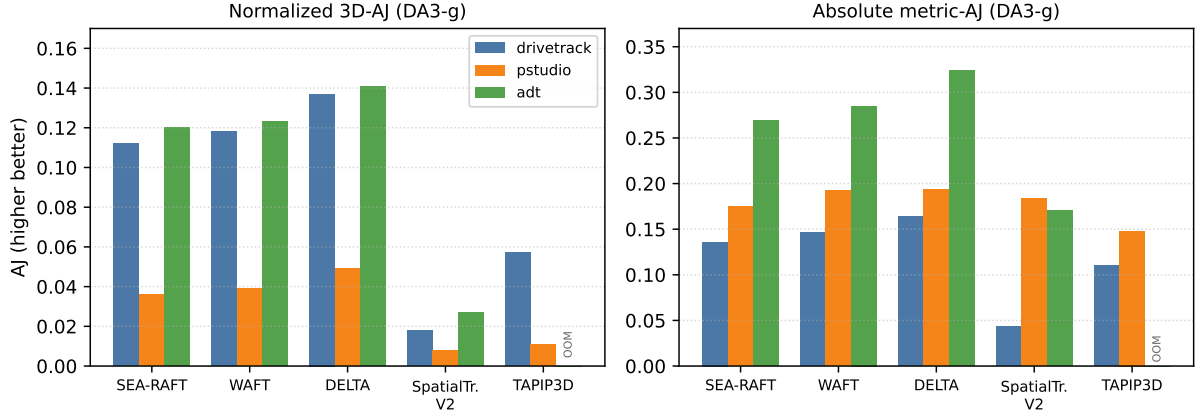
Figure 8: External baselines on DA3-g depth, per subset: normalized 3D-AJ (left) and absolute metric-AJ (right). Compared with Fig. 7, drivetrack metric-AJ jumps for every direct-unprojection method while the normalized metric is nearly unchanged; TAPI3D adt is OOM-limited.
