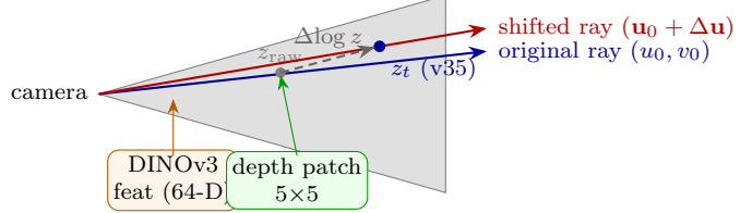
New SSM inputs (orange/green) \Rightarrow informed \Delta \mathbf{u} avoids depth-discontinuity artefacts. Depth is re-sampled at \mathbf{u}_0 + \Delta \mathbf{u} before applying \Delta \log z
