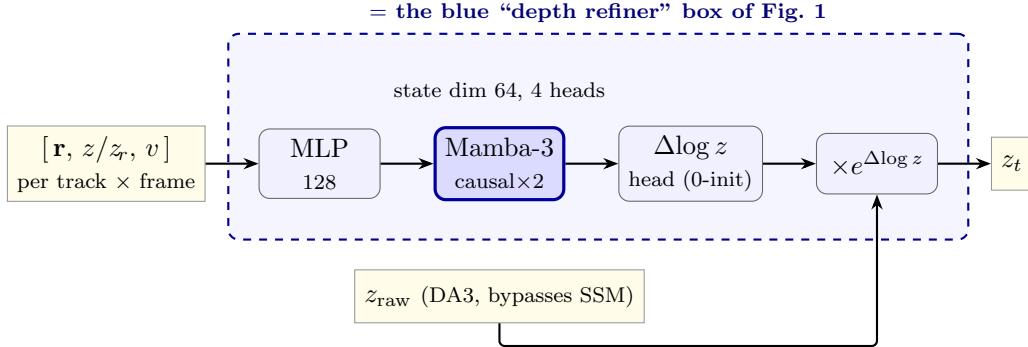
Figure 3: v33 architecture — the inside of the blue box in Fig. 1. Input abbreviations: \mathbf{r}=(\text{ray}_x, \text{ray}_y) is the frozen pixel ray from the 2D track \mathbf{u}_t , z/z_r=z_{\text{raw}}/z_{\text{ref}} , v =visibility. Bypass: z_{\text{raw}} (DA3 metric depth) skips the SSM entirely and is multiplied back in at the end — the SSM is a relative corrector that predicts the factor e^{\Delta \log z} , not an absolute depth. causal \times 2 : two causal Mamba-3 layers (past-only; enables streaming). 4 heads: SSD splits the 64-dim state into 4 independent heads (16-dim each), analogous to multi-head attention but computed as a linear recurrence.
