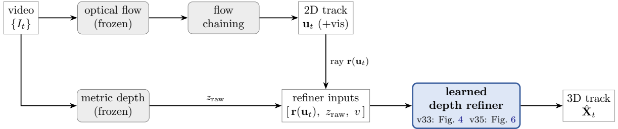
Figure 2: Overall pipeline. The flow front-end (SEA-RAFT or WAFT) and metric-depth backbone (DA3-l or DA3-g) are both frozen and swappable across this report’s experiments. Grey = frozen / training-free; the large blue box is the only learned module (0.40M params); its internals are Fig. 4 (v33) and Fig. 6 (v35). The frozen flow front-end’s 2D track \mathbf{u}_t (and visibility) is never modified. The refiner’s inputs (white box) — the frozen pixel ray \mathbf{r}(\mathbf{u}_t) (from \mathbf{u}_t and the intrinsics), the frozen depth backbone’s raw depth z_{\text{raw}} , and visibility v — are exactly the white input boxes that sit outside the blue box in Fig. 4 and Fig. 6 (v35 additionally feeds a 5 \times 5 depth patch and a DINOv3 feature). The box corrects depth along the frozen ray and unprojects to 3D, so the 2D reprojection is invariant by construction (Fig. 3).
