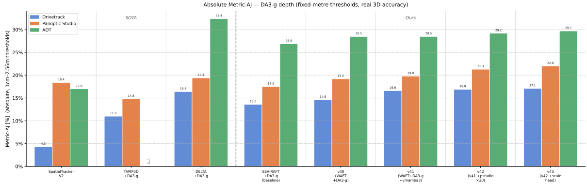
Figure 12: Method comparison on DA3-g depth, absolute metric-AJ (fixed-metre thresholds; higher better). Drivetrack rises across the board vs. DA3-l (Fig. 10), but pstudio/adtt do not, so even v42 — our best DA3-g pipeline (mean 0.225), which adds a pstudio \times 20 near-boost over v41 — does not beat the DA3-l v39 overall (0.246). TAPIP3D adtt is OOM-limited (“N/A”).
