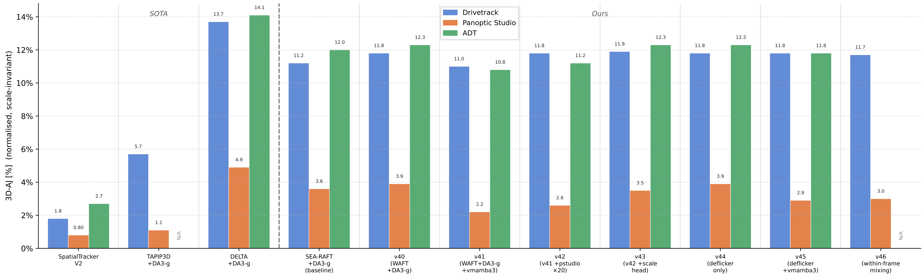
TAPVid-3D Normalised Median-AJ — DA3-g depth (higher = better)
