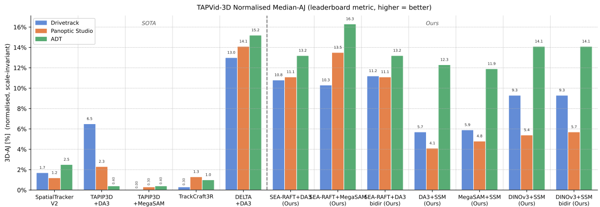
Figure 8: Method comparison on TAPVid-3D minival, normalised median-AJ (leaderboard metric, scale-invariant). Higher is better. “bidir” = bidirectional SEA-RAFT flow (reversed-video backward pass). TrackCraft3R’s low drivetrack bar reflects an OOD failure (see §2.4).
