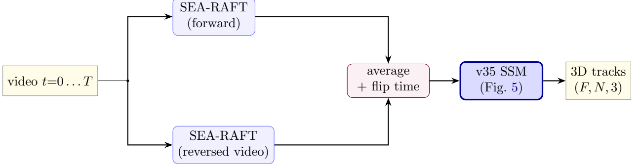
Figure 6: v36 pipeline. The v35 SSM is unchanged; SEA-RAFT runs on both the original and the time-reversed video, the two 2D track estimates are averaged (and the reversed-video result is flipped back to forward time), then passed to v35 as the starting 2D positions. Bidirectional flow improves coverage of points that are temporarily occluded in the forward direction but visible in the backward pass.
