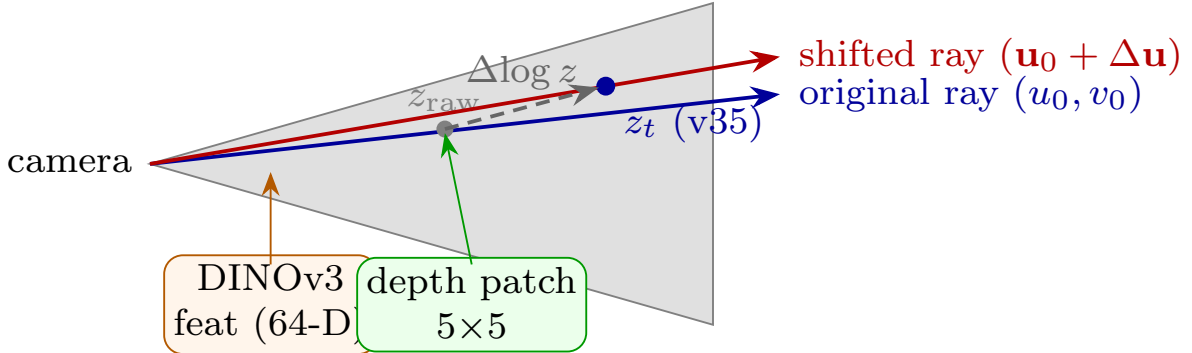
Figure 4: v35 joint correction. Two new inputs — the DINOv3 appearance feature (orange) and a local 5\times 5 depth patch (green) — give the SSM the context to predict a 2D shift \Delta \mathbf{u} safely. Unlike v32, which nudged the pixel blindly and crossed depth discontinuities, v35’s 2D correction is conditioned on local appearance and local depth structure, so the informed \Delta \mathbf{u} avoids depth-discontinuity artefacts. Depth is then re-sampled at the shifted pixel \mathbf{u}_0 + \Delta \mathbf{u} before e^{\Delta \log z} rescales it.
