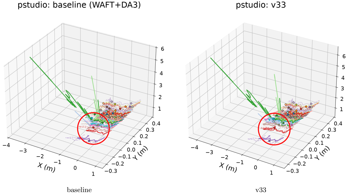
Figure 14: pstudio (indoor, ~3m), best clip basketball_3 : predicted (solid) vs ground-truth (dashed) 3D trajectories, baseline (left) vs our refiner v33 (right). Inside the red circle — the track our refiner corrects the most — v33’s solid path sits closer to the dashed ground truth than the baseline’s, i.e. the refiner improves the mid-range metric depth.
