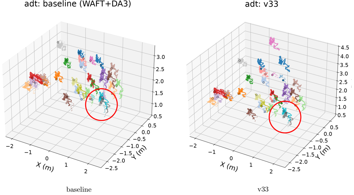
Figure 16: adt (egocentric, \sim 1 m), best clip Apartment_release_meal_seq136.8 : near-field, where DA3-l depth is already accurate. Predicted (solid) vs ground-truth (dashed), baseline (left) vs v33 (right). The red circle marks the most-corrected track; here the baseline is already close, so the refiner’s improvement is small (consistent with the near-field tie in Fig. 11) — crucially, it does not degrade the already-good near-field estimate.
