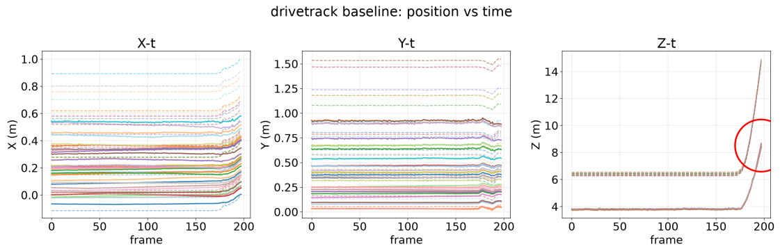
Figure 17: Space-time view (drivetrack baseline): per-axis position over time, X - t / Y - t / Z - t , predicted (solid) vs ground truth (dashed). X and Y track the ground truth well; the error lives almost entirely in Z (depth). The red circle on the Z - t panel marks the largest baseline depth error — the along-ray depth blow-up on the receding far point — which is exactly the failure our depth refiner is built to correct (cf. the circled regions in Figs. 15).
