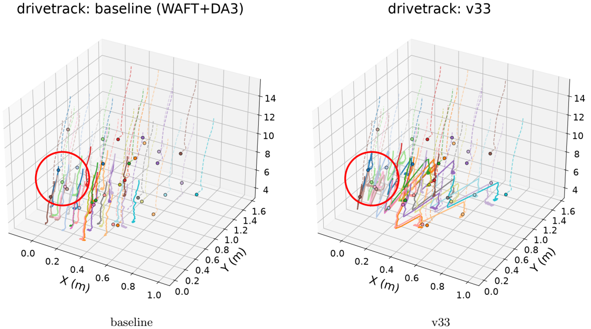
Figure 15: drivetrack (driving, ~20m), best clip: the far-field scene where our refiner helps most. Predicted (solid) vs ground-truth (dashed), baseline (left) vs v33 (right). Inside the red circle , the baseline squashes the far tracks toward the camera (solid short of the dashed ground truth); v33 stretches them back out to the correct metric depth, closing most of the gap — this is the single biggest source of our absolute-metric-AJ win on drivetrack.
