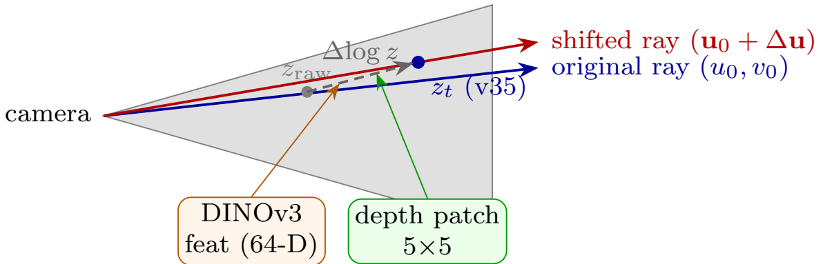
Figure 4: v35 joint correction. Two new inputs — the DINOv3 appearance feature (orange) and a local 5\times 5 depth patch (green) — give the SSM the context to predict a 2D shift \Delta\mathbf{u} safely. Unlike v32, which nudged the pixel blindly and crossed depth discontinuities, v35’s 2D correction is conditioned on local appearance and local depth structure, so the informed \Delta\mathbf{u} avoids depth-discontinuity artefacts. Depth is then re-sampled at the shifted pixel \mathbf{u}_0 + \Delta\mathbf{u} before e^{\Delta\log z} rescales it.
