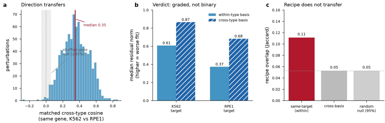
Figure S7: Cross-cell-type transfer: direction transfers, the minimal recipe does not. The unchanged operator applied to the Replogle et al. [15] K562 and RPE1 essential-gene screens (843 shared perturbations, 2,832 shared genes). (a) A single perturbation's effect direction transfers moderately (matched cross-type cosine median 0.35; grey band, shuffled-gene null \pm 95\% ). (b) The reachability verdict transfers only as a graded residual: the median residual norm is systematically worse under a cross-type basis (hatched) than a within-type basis, for both K562 and RPE1 targets. (c) The minimal recipe does not transfer—same-target Jaccard overlap (0.11) collapses toward the random-selection null (0.05) under a cross-type basis. Direction is portable across cell types; the specific recipe is not.
