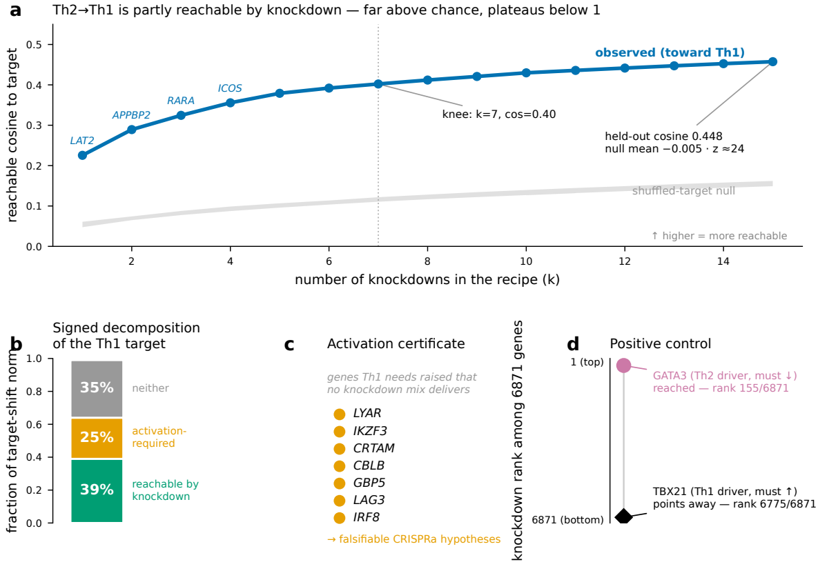
Figure 2: T_H2 \rightarrow T_H1 is partly reachable by knockdown. (a) Greedy reachability spectrum: reachable cosine versus recipe size k , far above the shuffled-target null at every k , with a knee at k = 7 (cosine 0.40) and a held-out cosine of 0.448 (null mean -0.005 , z \approx 24 ). (b) Signed decomposition of the target: 39% reachable by knockdown, 25% activation-required, 35% neither. (c) Activation certificate: seven genes the T_H1 target needs raised that no knockdown mix supplies—falsifiable CRISPRa hypotheses. (d) Positive control: the T_H2 driver GATA3 is reached (rank 155/6871) while the T_H1 driver TBX21 is correctly anti-aligned (rank 6775/6871).
