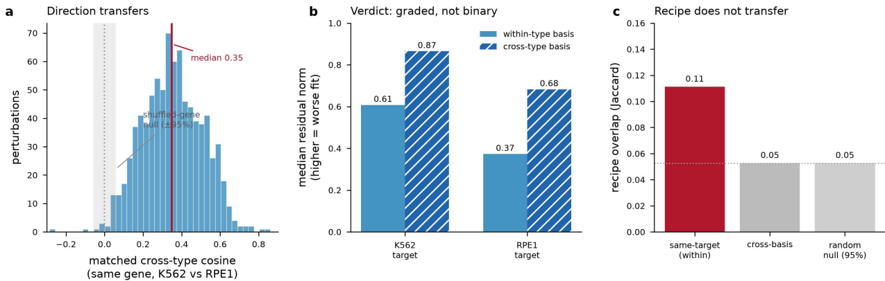
Figure S7. Cross-cell-type transfer: direction transfers, the greedy recipe does not. The unchanged operator applied to the Replogle et al. (2022) K562 and RPE1 essential-gene screens (843 shared perturbations, 2,832 shared genes). (a) A single perturbation's effect direction transfers moderately (matched cross-type cosine median 0.35; grey band, shuffled-gene null ±95%). (b) The reachability verdict transfers only as a graded residual: the median residual norm is systematically worse under a cross-type basis (hatched) than a within-type basis, for both K562 and RPE1 targets. (c) The greedy recipe does not transfer—same-target Jaccard overlap (0.11) collapses toward the random-selection null (0.05) under a cross-type basis. Direction is portable across cell types; the specific recipe is not.
