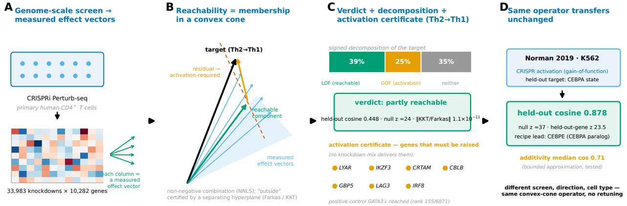
Figure 1. The convex-cone reachability oracle. (A) A genome-scale CRISPRi Perturb-seq screen in primary human CD4 + T cells yields 33,983 perturbation–condition effect profiles over 10,282 genes, filtered to 6,871 generators for the resting analysis. (B) Reachability is membership in the non-negative conic hull of these vectors; the reachable component is the NNLS projection of the target, and the residual is the outside-the-cone direction, with “outside” certified by a separating hyperplane (Farkas/KKT). (C) For Th2→Th1 the oracle returns a partly reachable verdict (held-out cosine 0.448, \|KKT/Farkas\| \approx 1.1 \times 10^{-11} ), a signed decomposition (39% LOF / 25% GOF / 35% neither), and an dual certificate ranking positive unmet readouts. (D) The identical operator, with no retuning, transfers to the Norman K562 CRISPRa screen (held-out CEBPA cosine 0.878).
