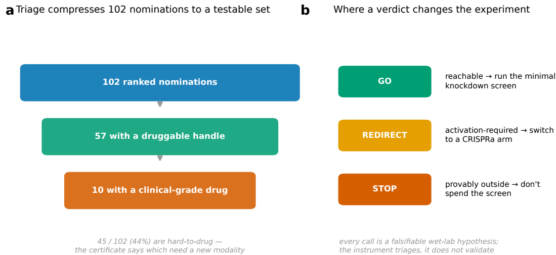
Figure S4. Triage funnel and the three actions a verdict enables. (a) The union of top-10 greedy LOF panels contains 102 unique candidates: 57 carry a druggable handle and 10 have a clinical-grade drug, while 45/102 (44%) are hard-to-drug. (b) Each state-level verdict maps to one action—GO (test a greedy sparse CRISPRi panel), REDIRECT (test the sign-flipped GOF hypothesis in a CRISPRa/de-repression arm), or STOP (no signal above the null; seek a different dictionary or modality). Candidate-level tractability annotations prioritize within the chosen arm. Every call is a falsifiable wet-lab hypothesis; the instrument triages, it does not validate.
