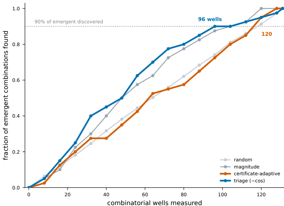
Certificate-adaptive acquisition does not beat a training-free score
